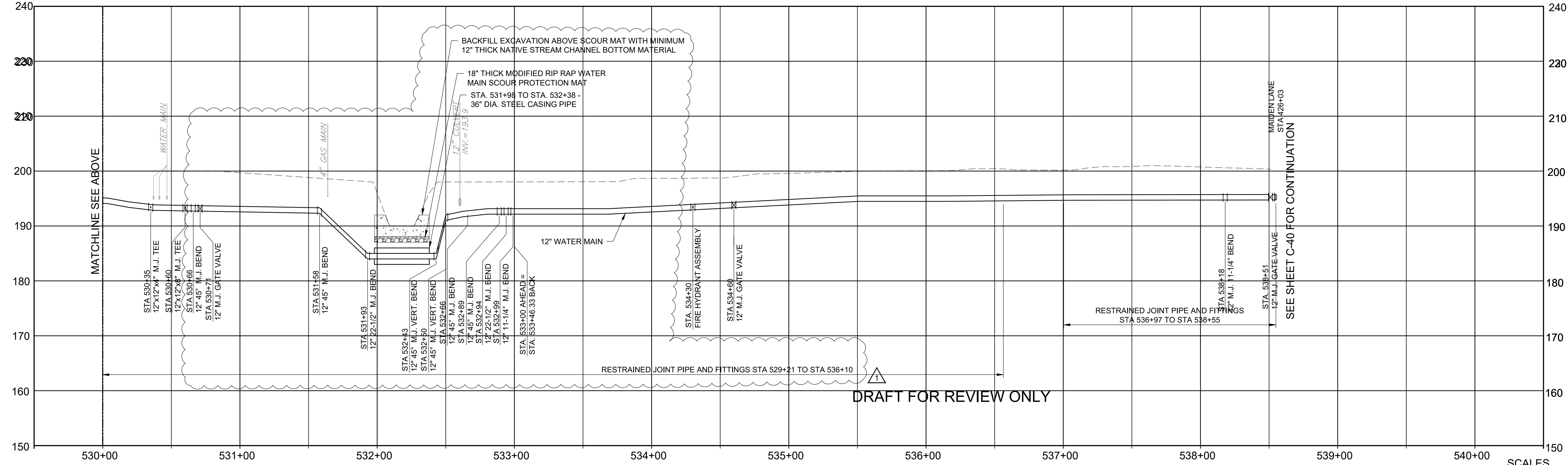
PICKETT LANE PROFILE VIEW STA. 530+00 TO STA. 538+55
