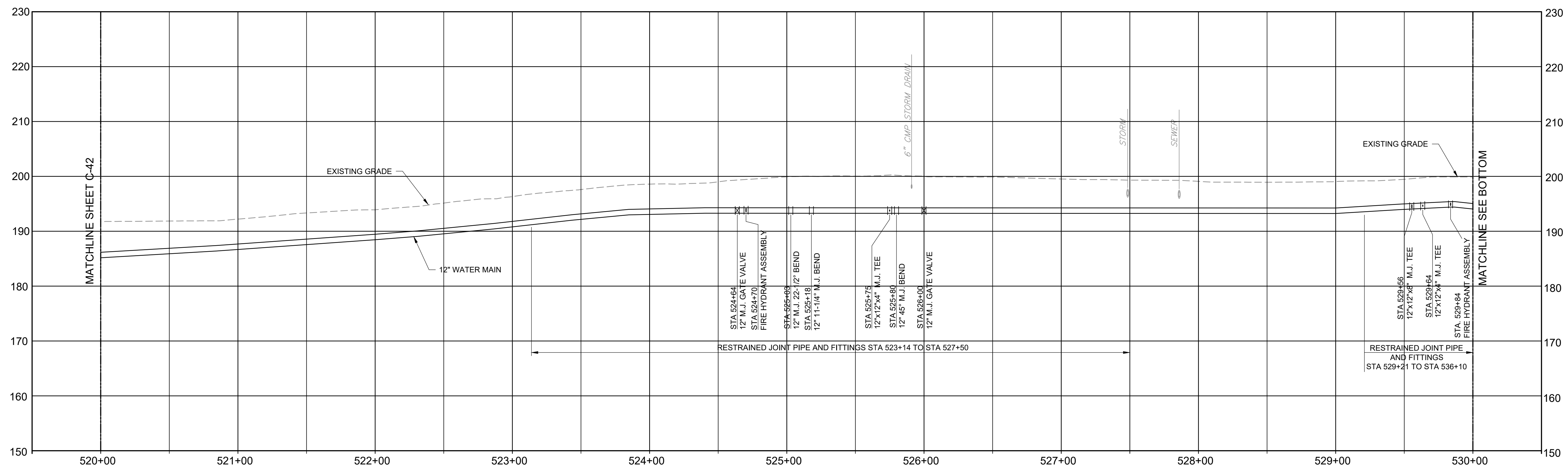
PICKETT LANE PROFILE VIEW STA. 520+00 TO STA. 530+00
